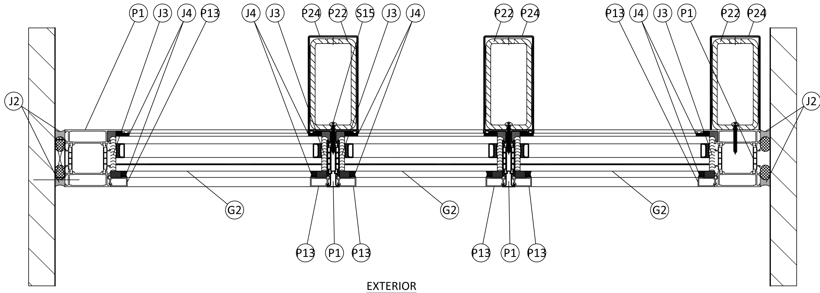
HORIZONTAL SECTION THROUGH FRAME - ANCHORED JAMB
